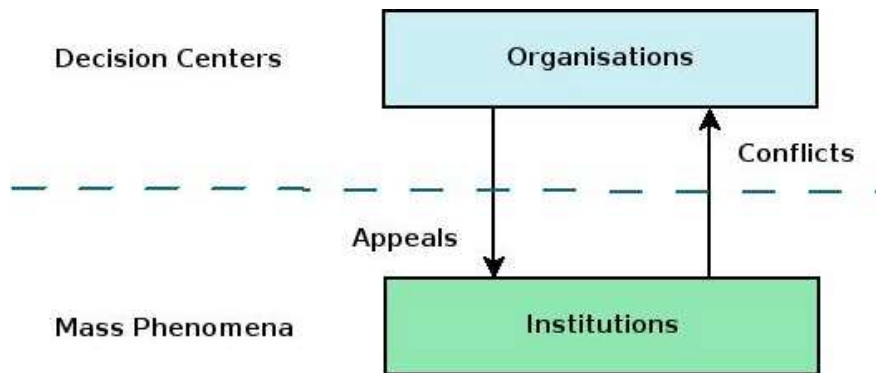
Figure 3: causal structure of the model intersection
