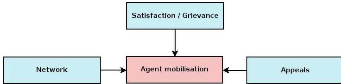
Figure 1: causal structure of agent's ethnic mobilisation
