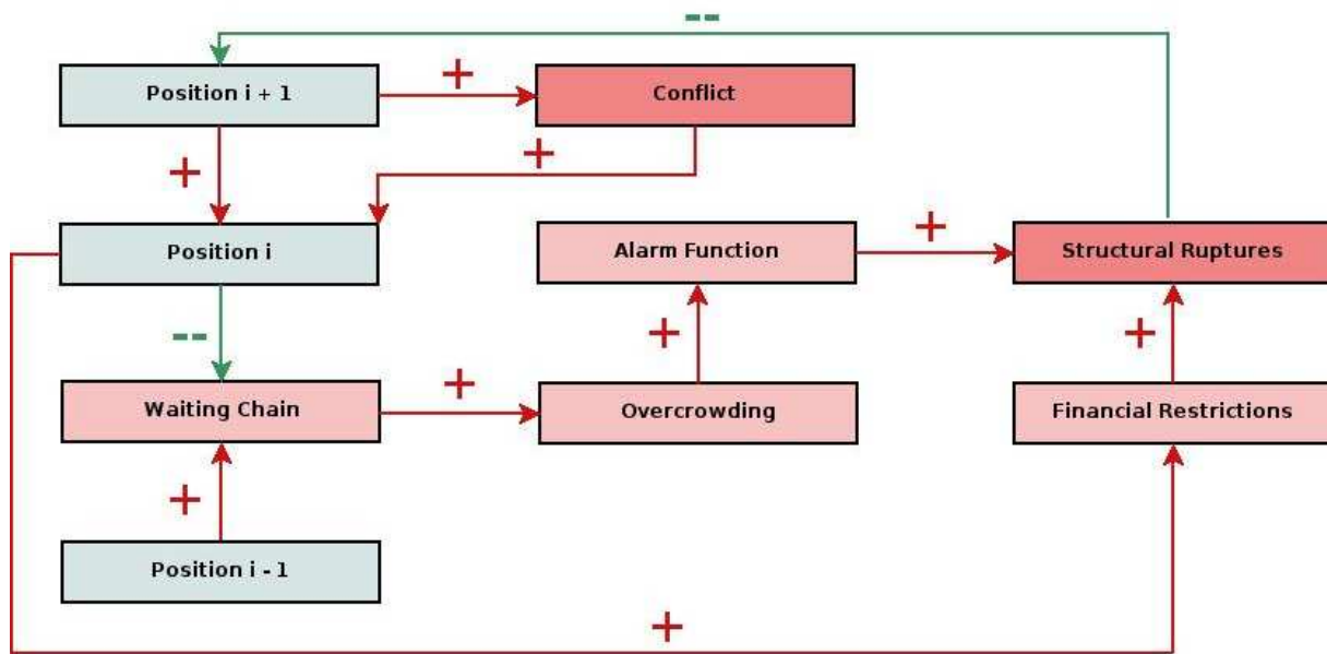
Figure 2: causal structure of the hierarchical operations
